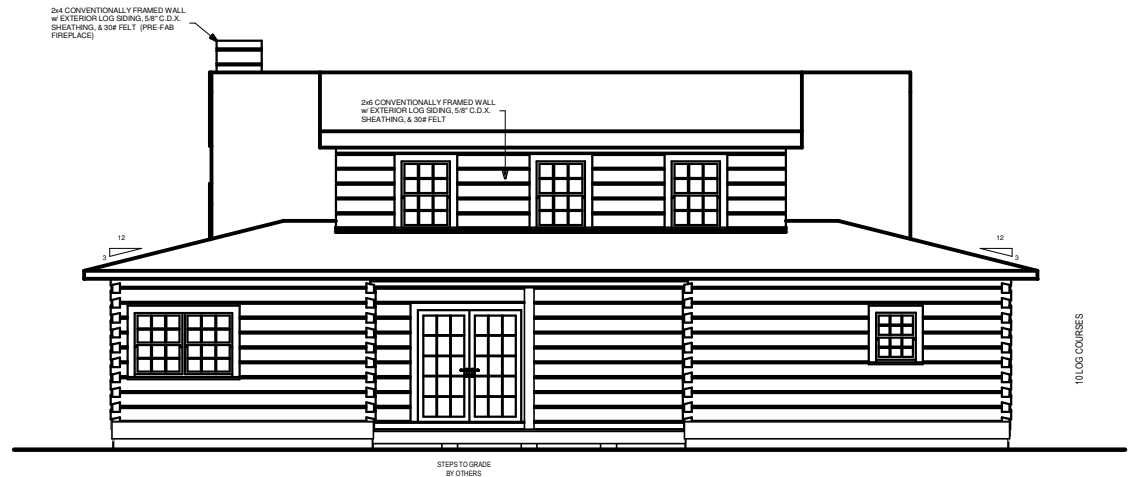
REAR ELEVATION
