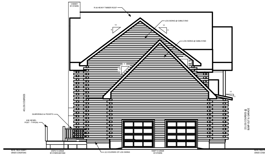
LEFT ELEVATION
