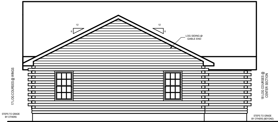
LEFT ELEVATION
