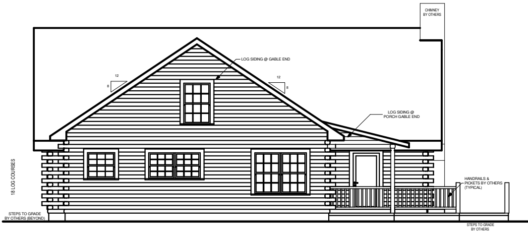
LEFT ELEVATION
