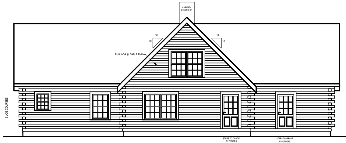
REAR ELEVATION
