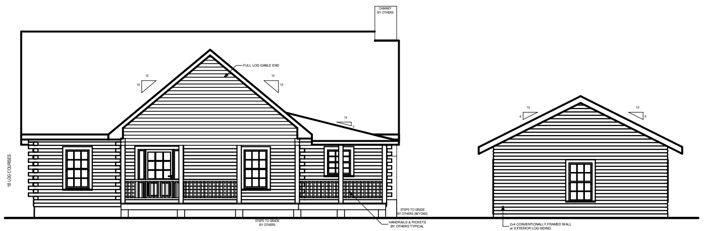
REAR ELEVATION
