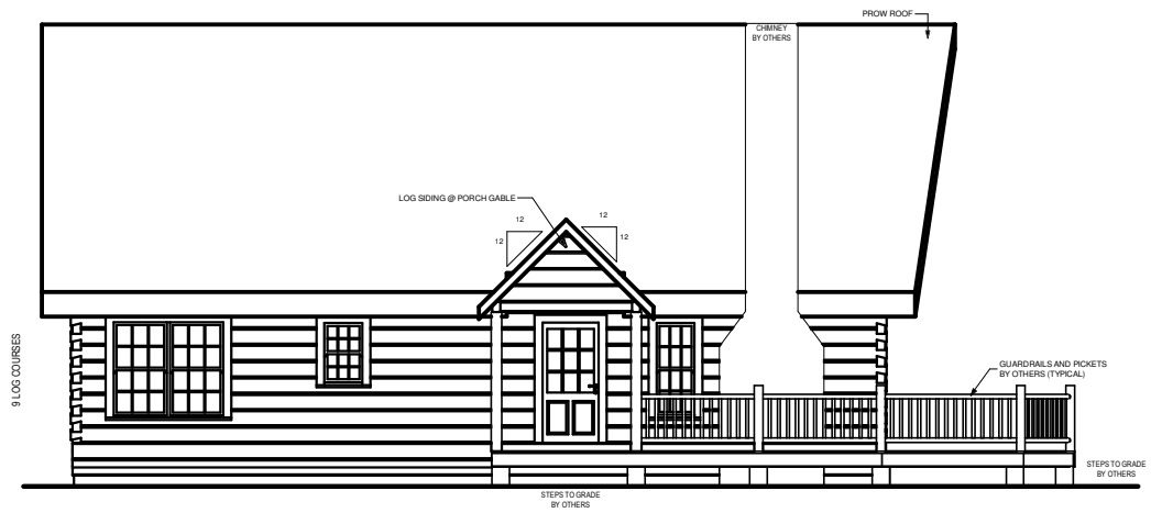
LEFT ELEVATION
