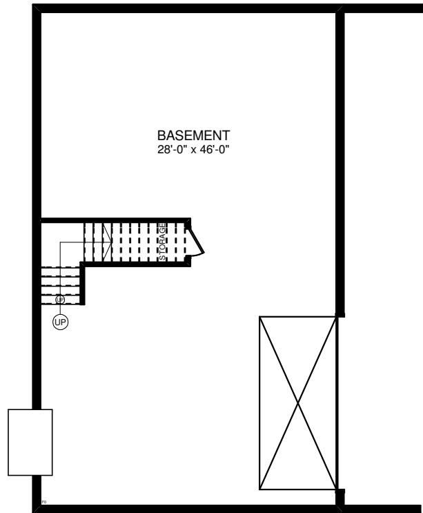
FOUNDATION PLAN
