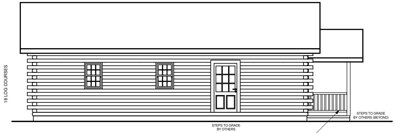
LEFT ELEVATION
