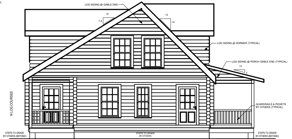
LEFT ELEVATION
