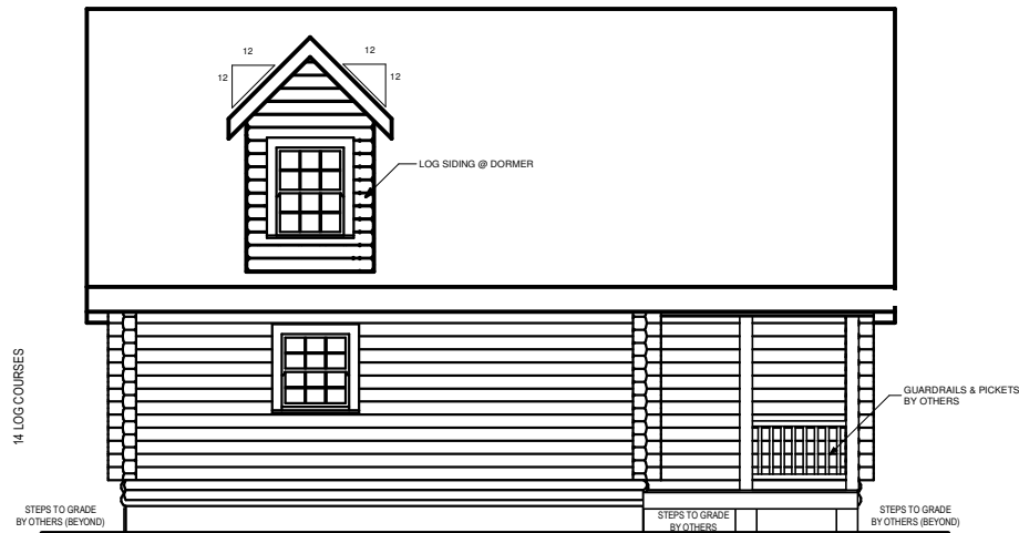
REAR ELEVATION
