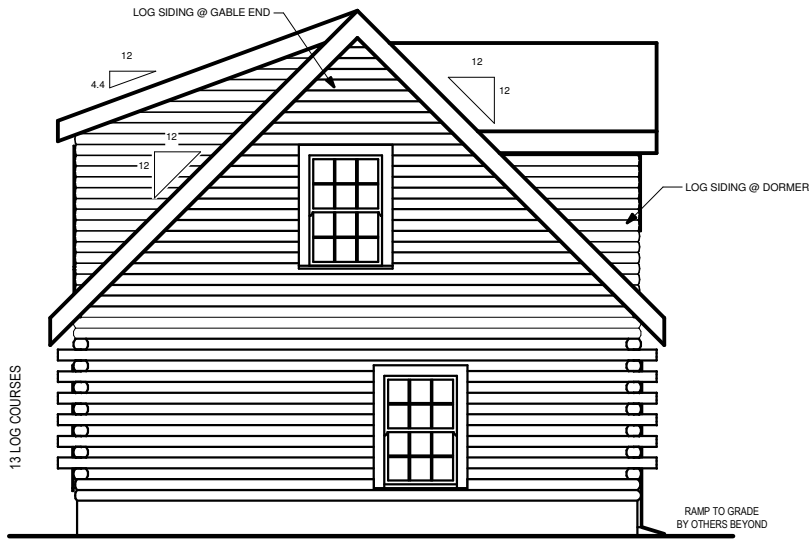
LEFT ELEVATION
