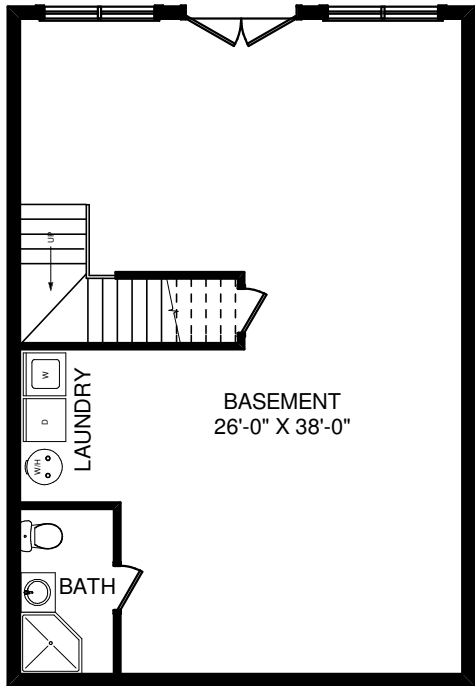
BASEMENT PLAN
