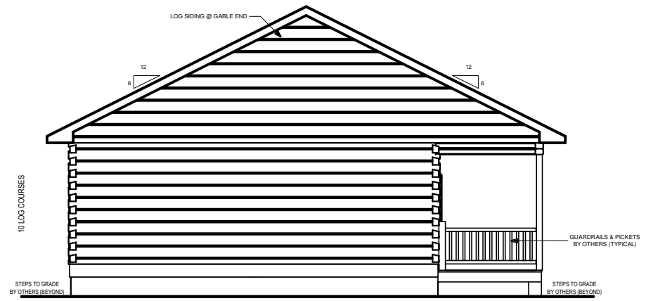
LEFT ELEVATION
