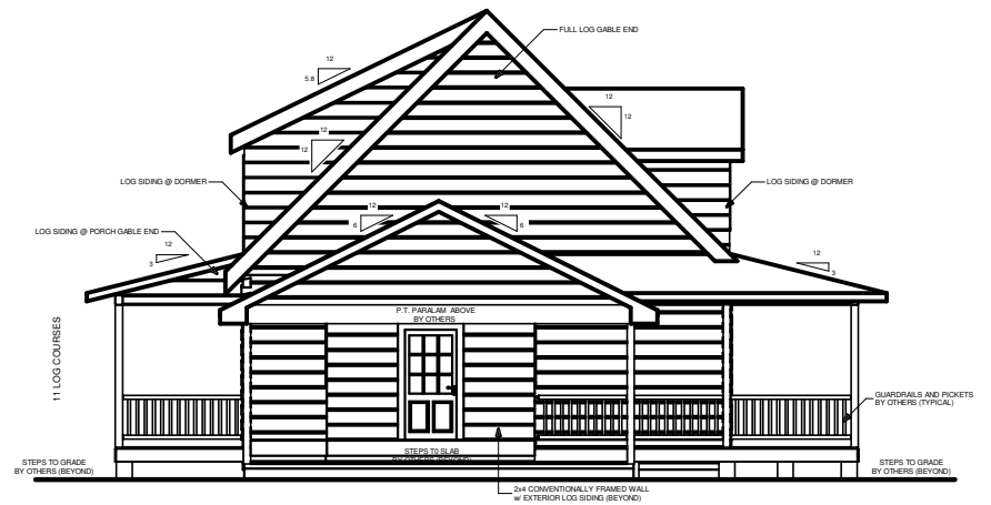
LEFT ELEVATION
