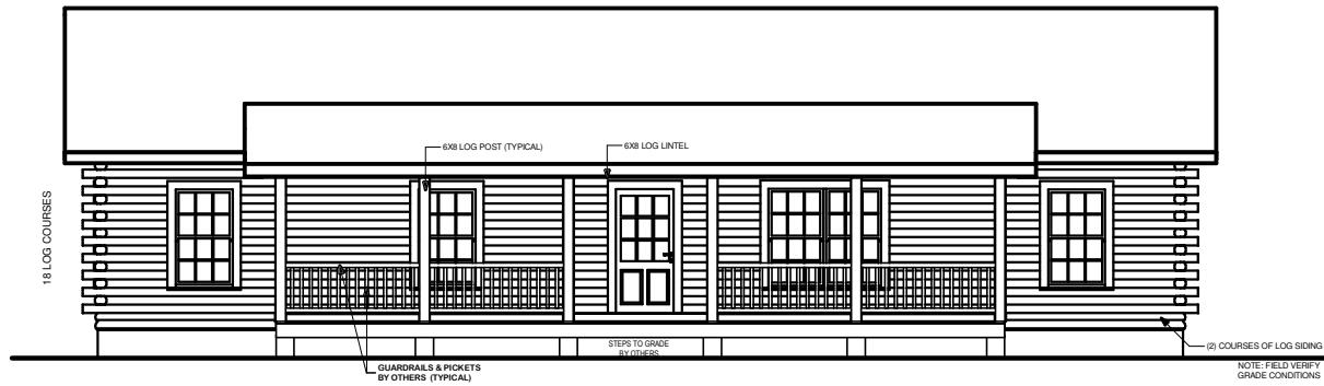
FRONT ELEVATION
