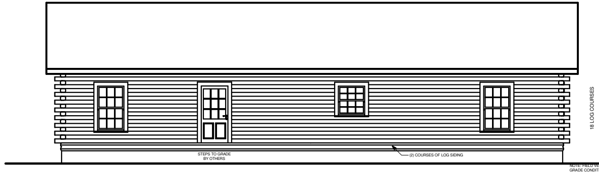
REAR ELEVATION
