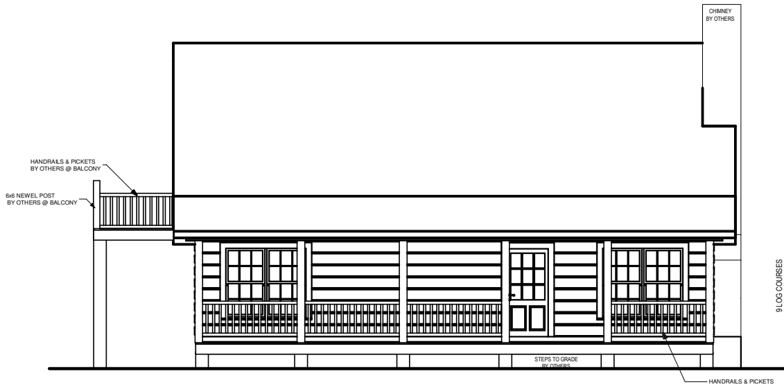
FRONT ELEVATION
