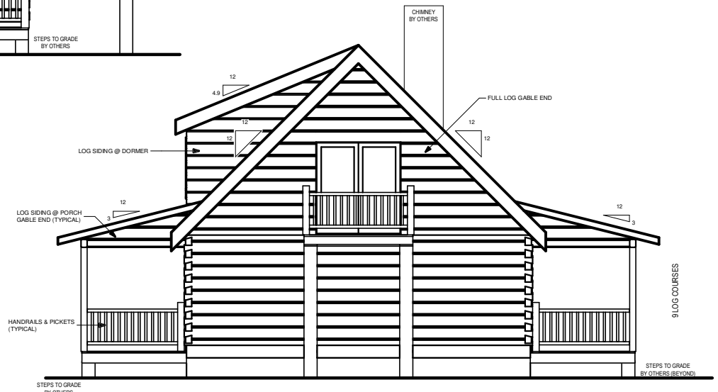
LEFT ELEVATION
