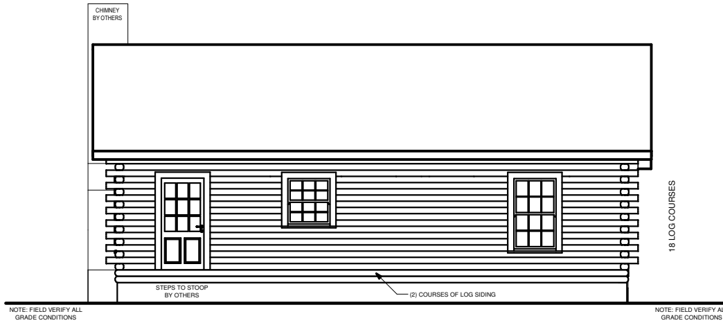
REAR ELEVATION
