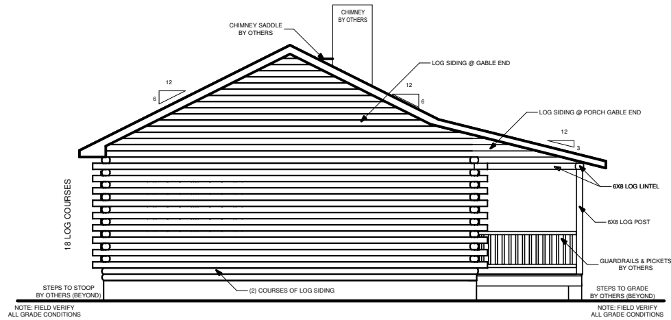
LEFT ELEVATION
