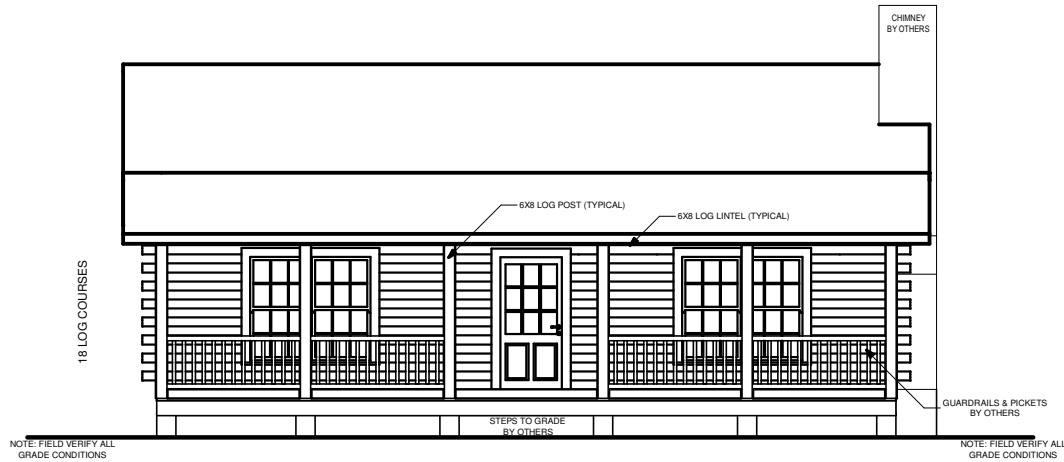
FRONT ELEVATION
