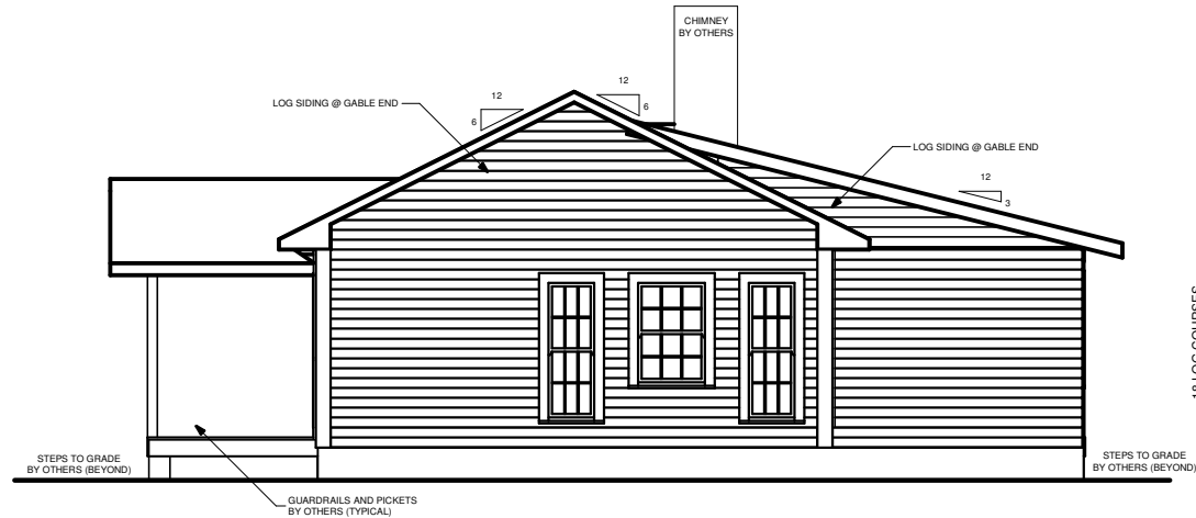
REAR ELEVATION
