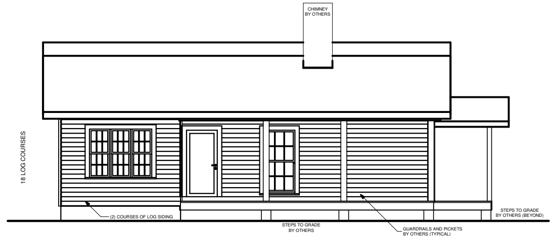
LEFT ELEVATION
