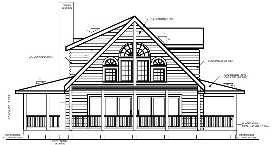
LEFT ELEVATION
