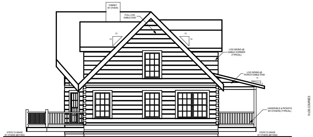
LEFT ELEVATION
