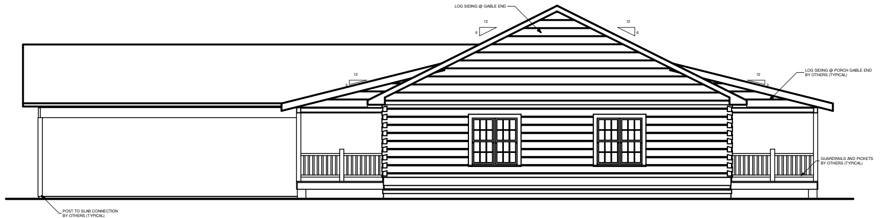
LEFT ELEVATION
