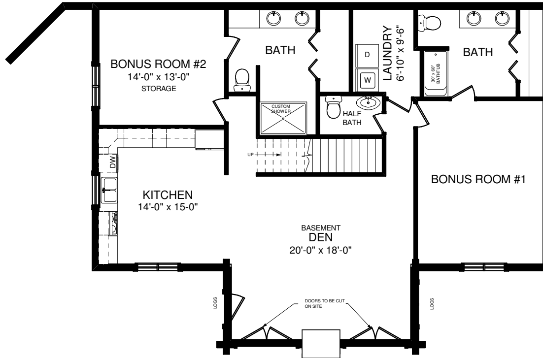
BASEMENT/ FOUNDATION PLAN
