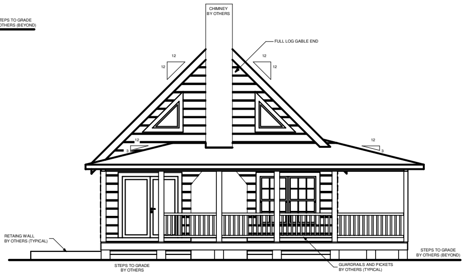
LEFT ELEVATION
