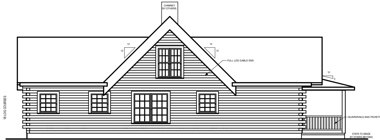
REAR ELEVATION
