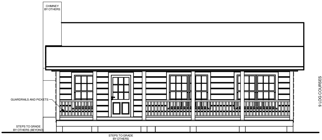
FRONT ELEVATION
