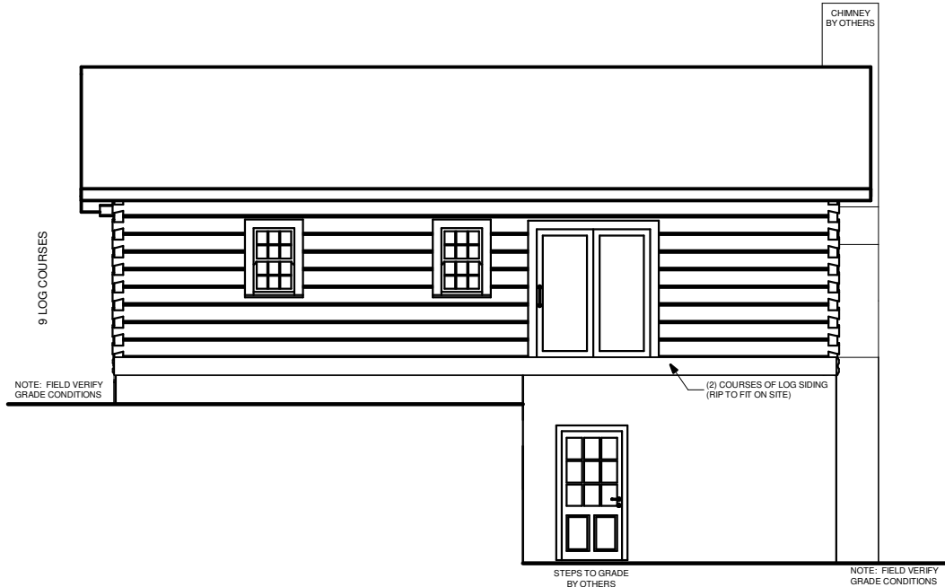
REAR ELEVATION
