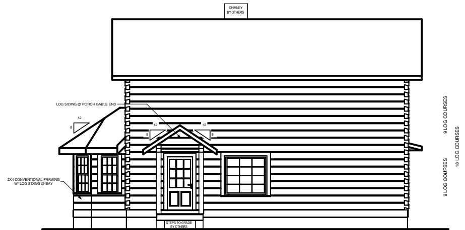
LEFT ELEVATION
