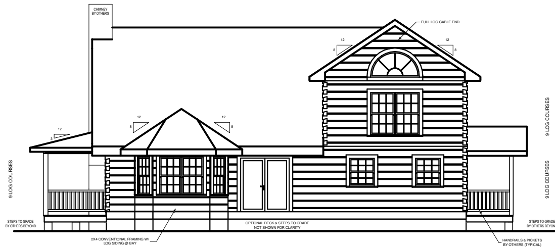
REAR ELEVATION
