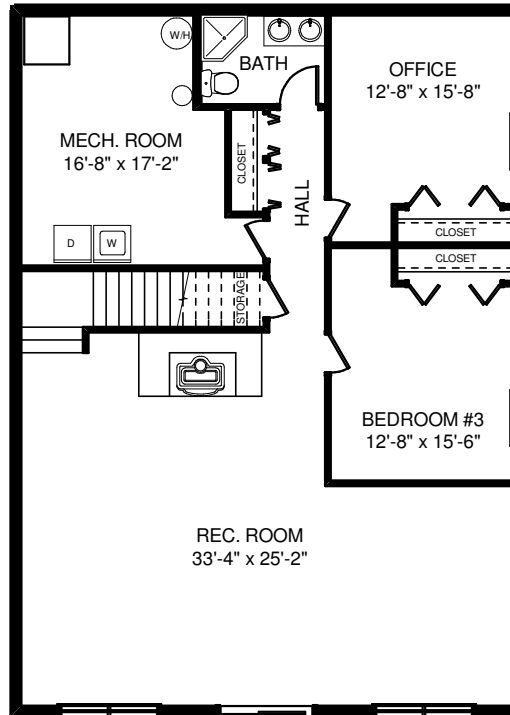
BASEMENT PLAN
