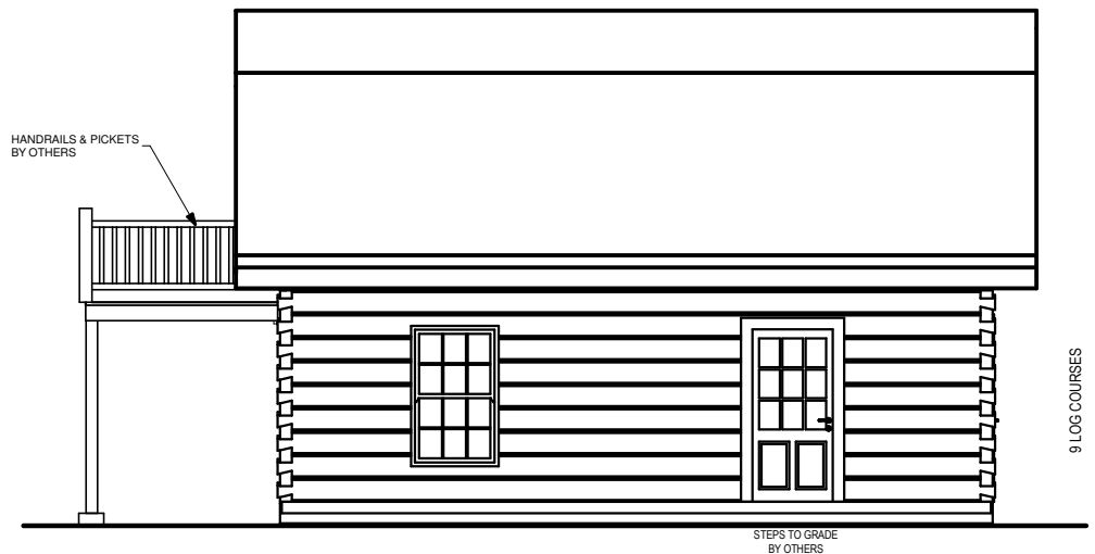
LEFT ELEVATION
