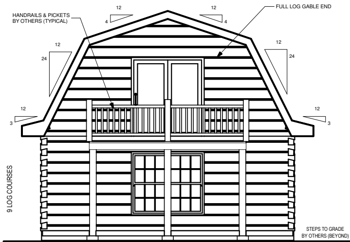
REAR ELEVATION
