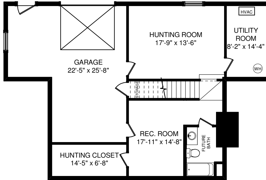
BASEMENT PLAN
