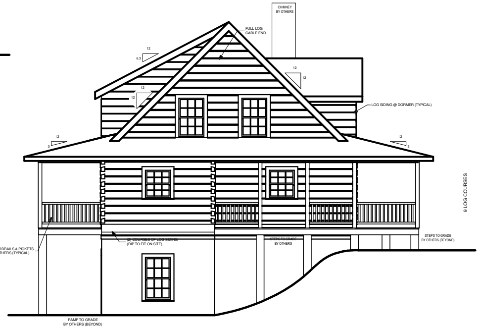
LEFT ELEVATION
