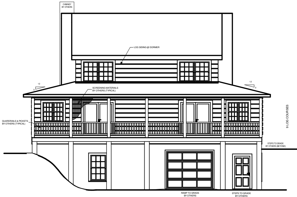
REAR ELEVATION
