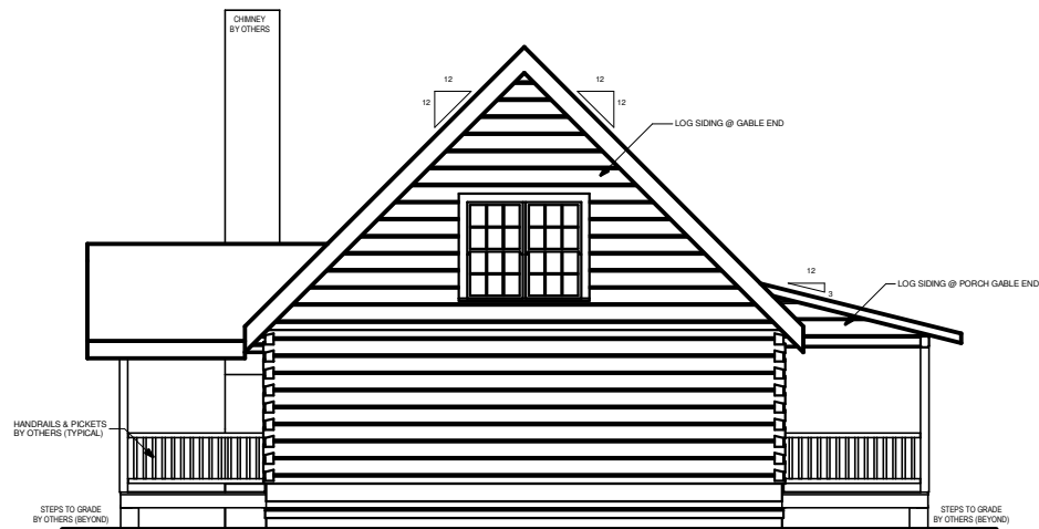
REAR ELEVATION
