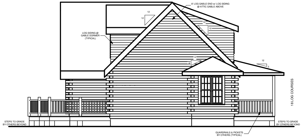
LEFT ELEVATION
