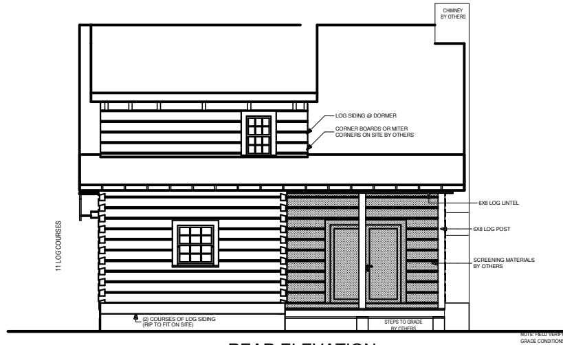
REAR ELEVATION
