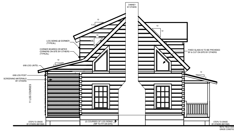
LEFT ELEVATION
