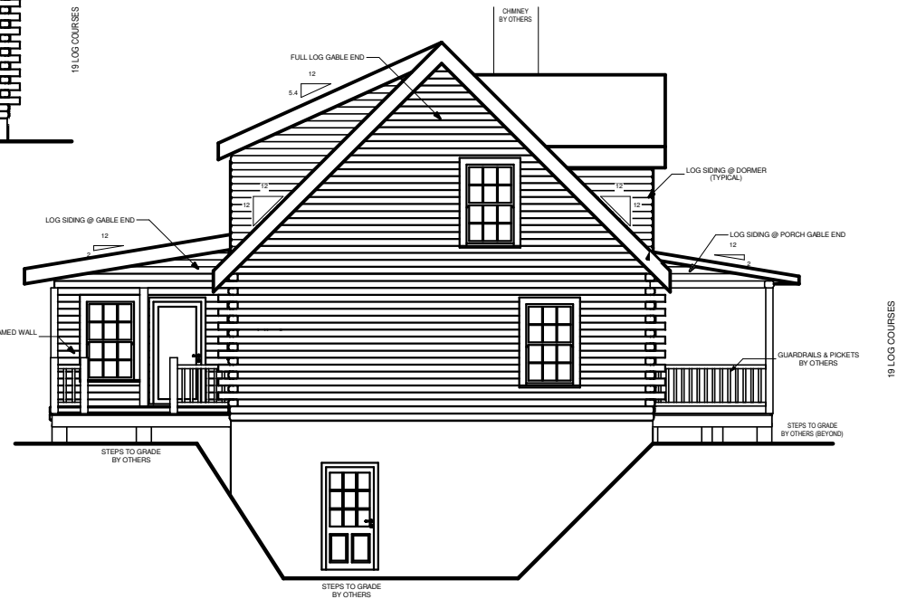
LEFT ELEVATION
