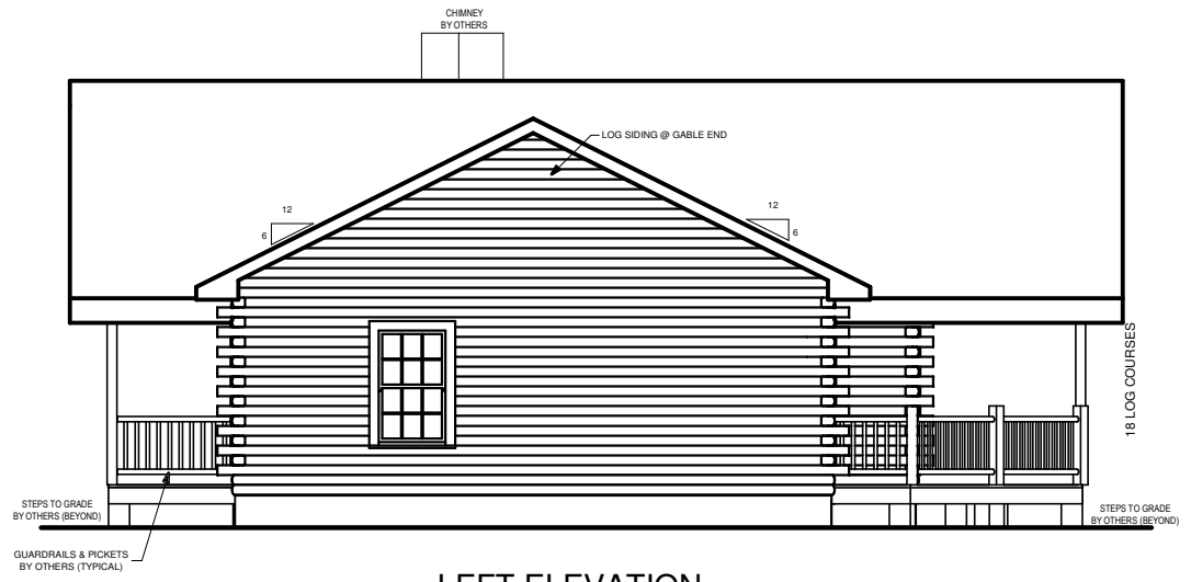
LEFT ELEVATION
