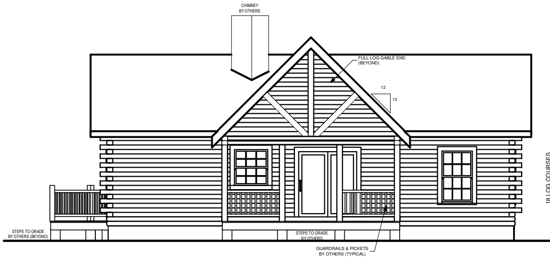
REAR ELEVATION
