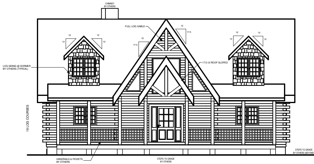
FRONT ELEVATION
