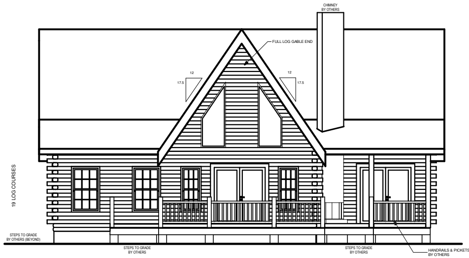
REAR ELEVATION
