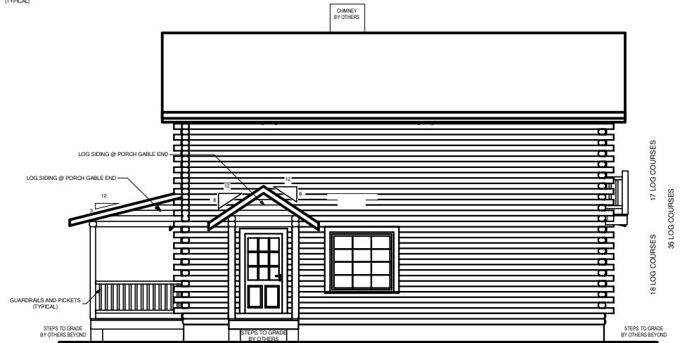
LEFT ELEVATION
