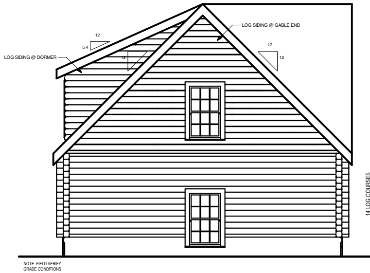
REAR ELEVATION
