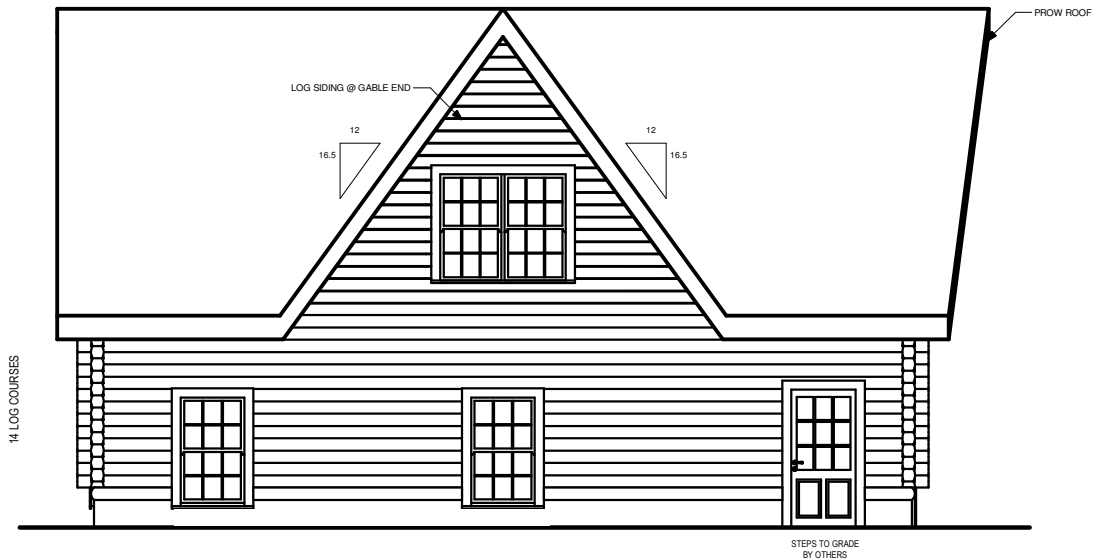
LEFT ELEVATION
