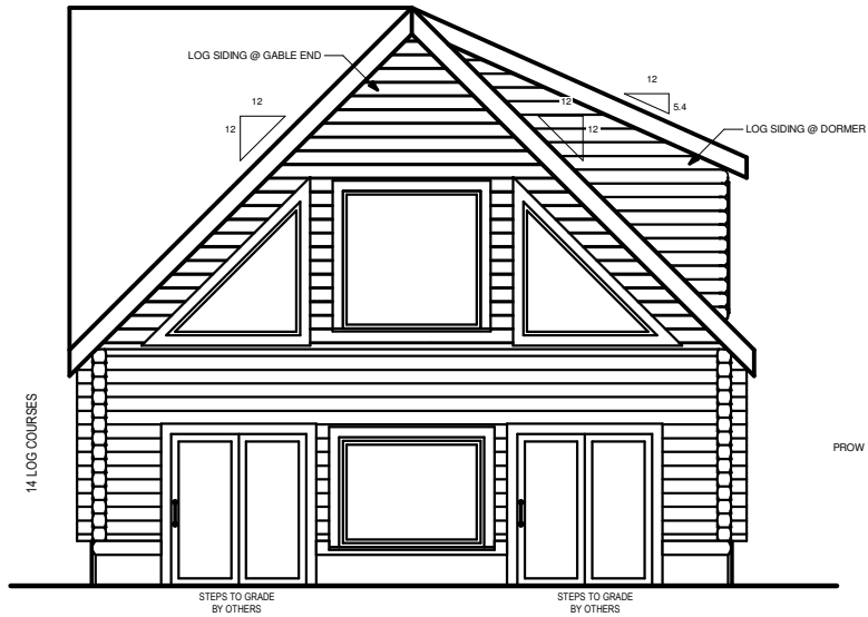
FRONT ELEVATION
