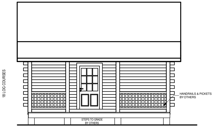
REAR ELEVATION
