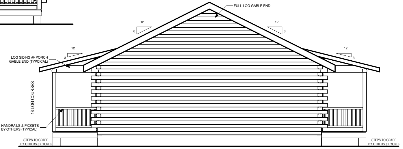
REAR ELEVATION
