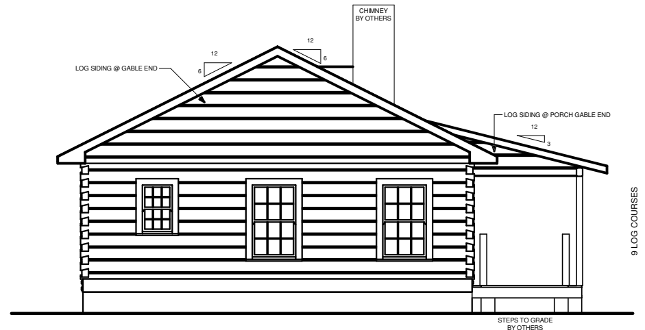
LEFT ELEVATION
