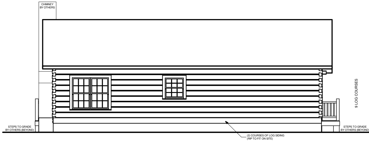
REAR ELEVATION
