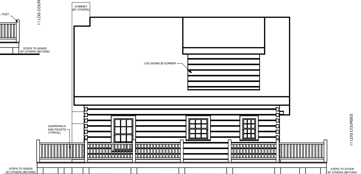
LEFT ELEVATION
