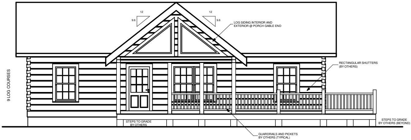
FRONT ELEVATION
