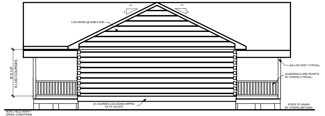
LEFT ELEVATION
