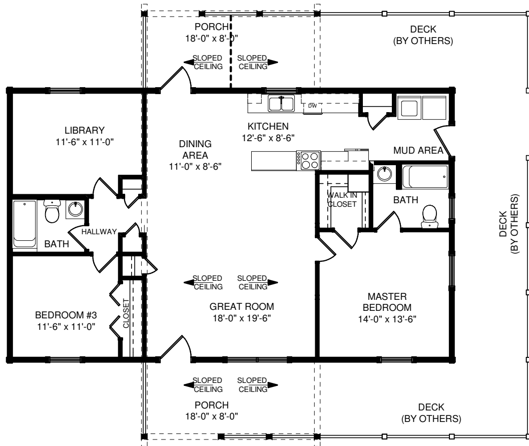
FLOOR PLAN 1/4" = 1'-0"
