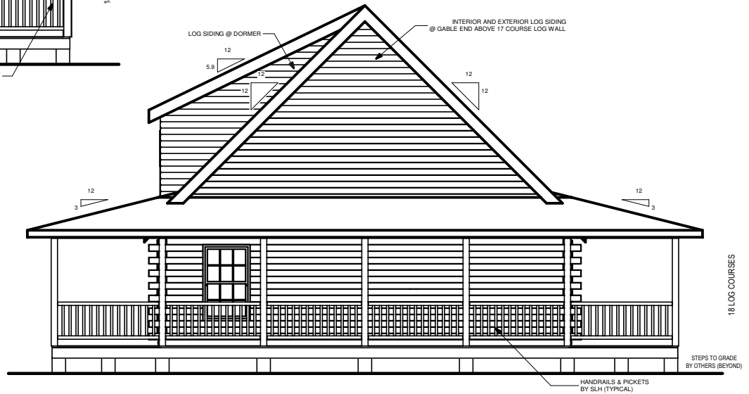
LEFT ELEVATION
