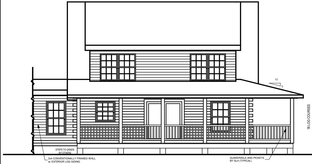
REAR ELEVATION
