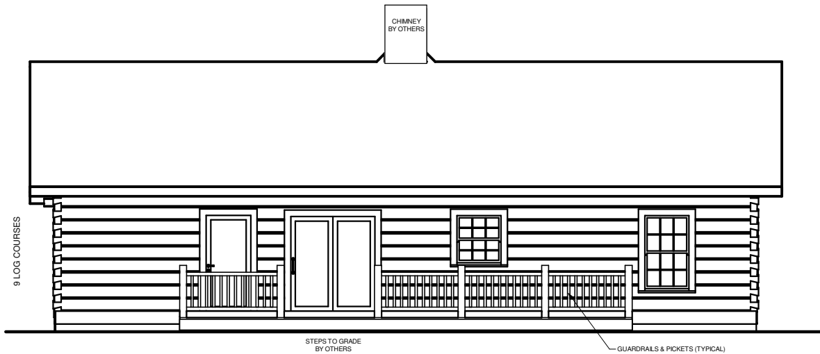
REAR ELEVATION
