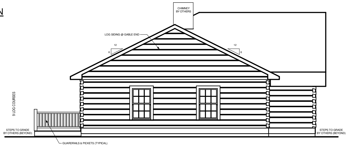
LEFT ELEVATION
