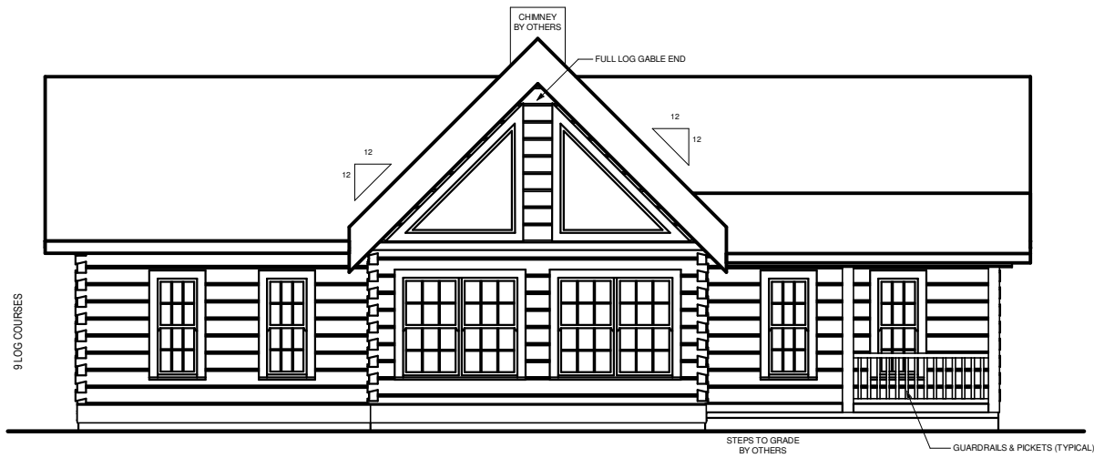
FRONT ELEVATION
