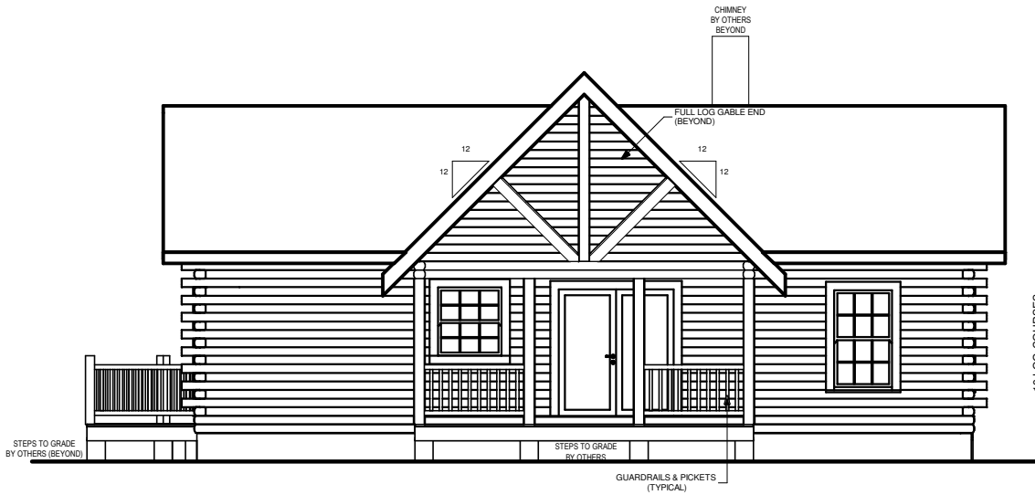
FRONT ELEVATION
