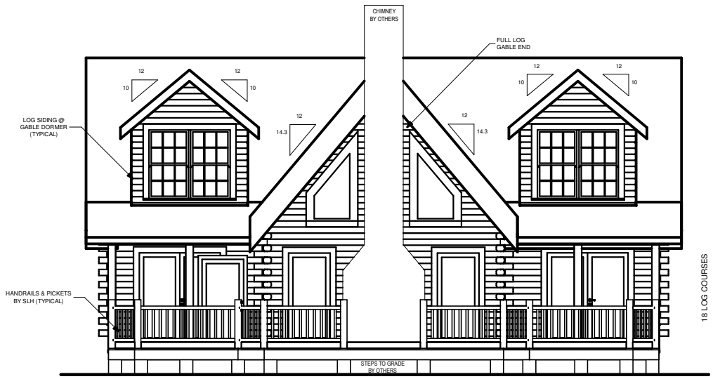
REAR ELEVATION
