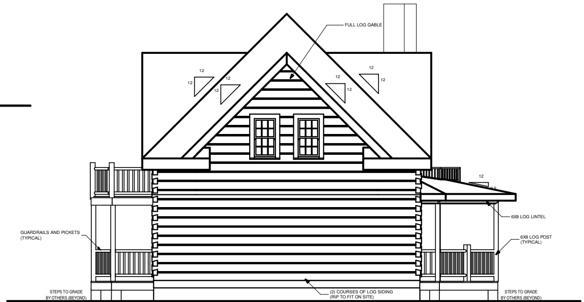
LEFT ELEVATION
