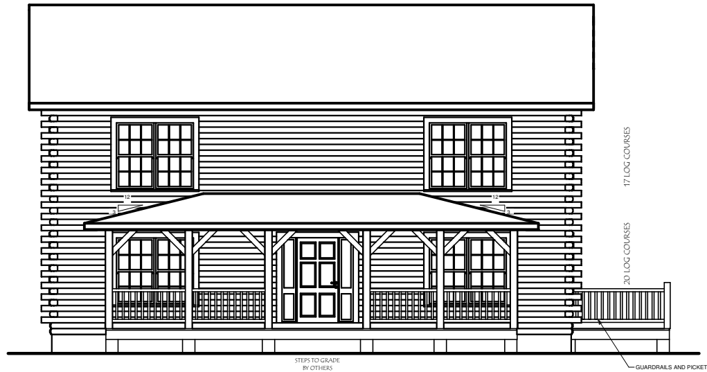
FRONT ELEVATION
