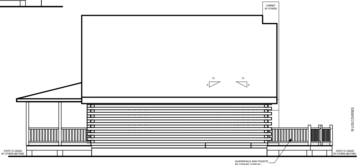
LEFT ELEVATION
