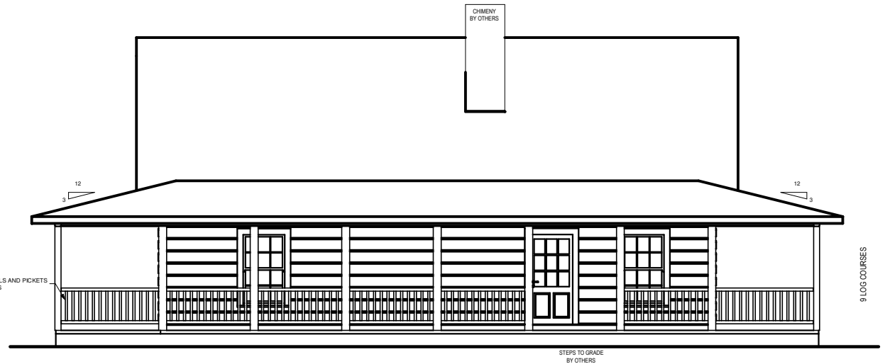
LEFT ELEVATION
