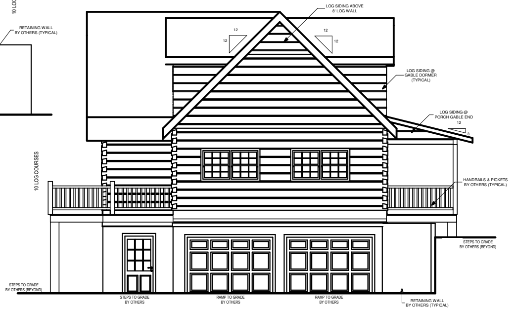
LEFT ELEVATION
