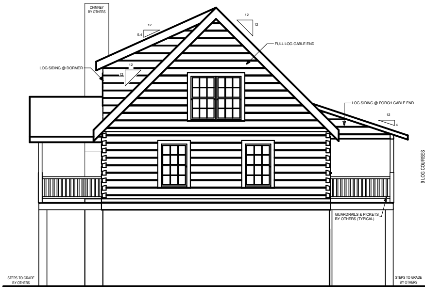
REAR ELEVATION
