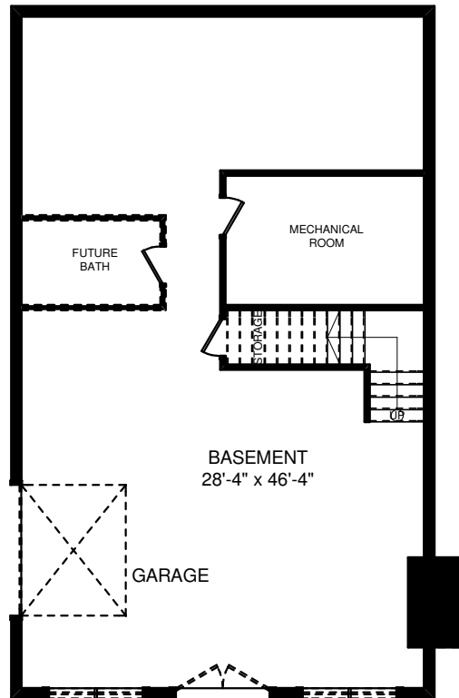
BASEMENT PLAN
