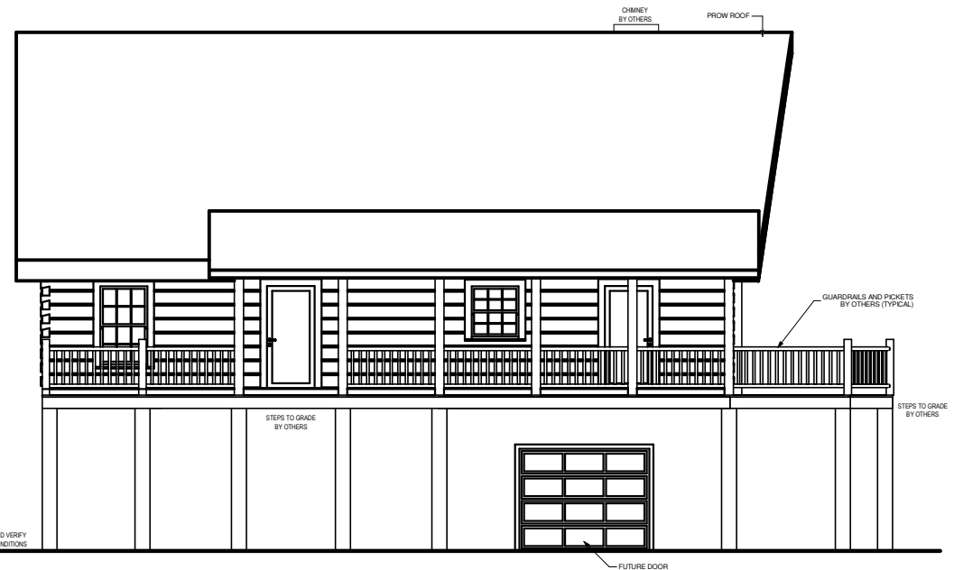
LEFT ELEVATION
