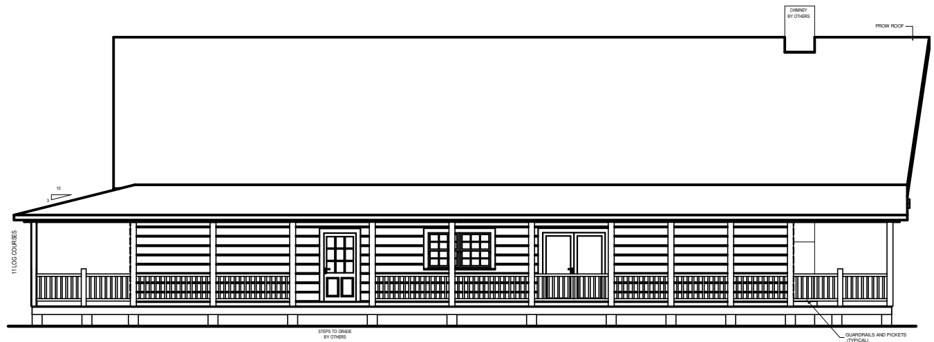
LEFT ELEVATION
